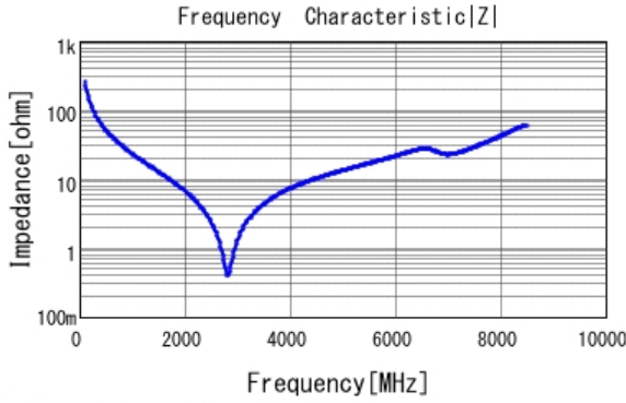
■ GCM1885C1H6R0CA16 |Z| DCOV, 25degC
