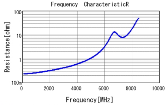
■ GCM1885C1H6R0CA16 R DCOV, 25degC
