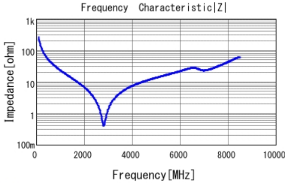
■ GCM1885C1H6R0DA16 |Z| DCOV, 25degC
