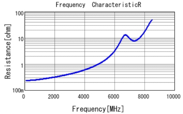
■ GCM1885C1H6R0DA16 R DCOV, 25degC
