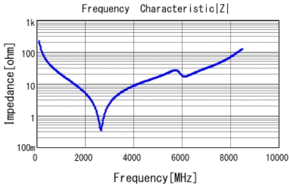
■ GCM1885C1H7R0DA16 |Z| DCOV, 25degC
