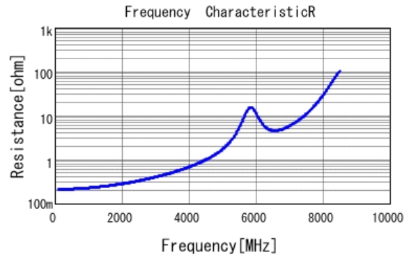
■ GCM1885C1H7R0DA16 R DCOV, 25degC
