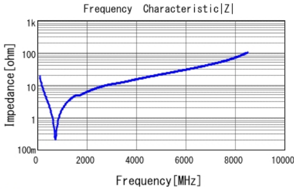
■ GCM1885C1H820JA16 |Z| DCOV, 25degC
