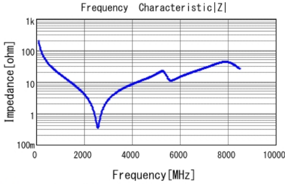
■ GCM1885C1H8R0BA16 |Z| DCOV, 25degC
