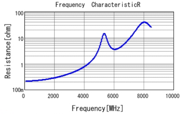
■ GCM1885C1H8R0BA16 R DCOV, 25degC
