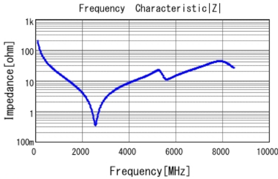
■ GCM1885C1H8R0CA16 |Z| DCOV, 25degC
