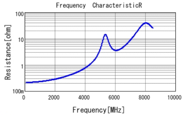
■ GCM1885C1H8R0CA16 R DCOV, 25degC
