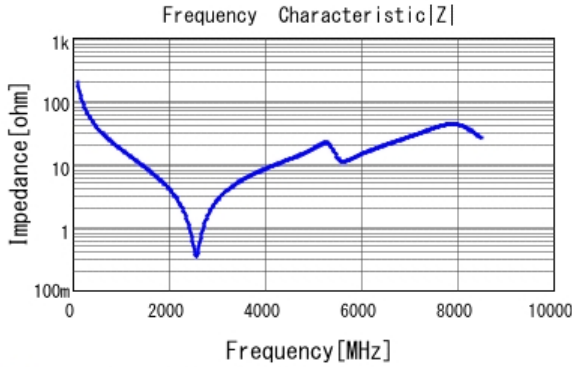
■ GCM1885C1H8R0DA16 |Z| DCOV, 25degC
