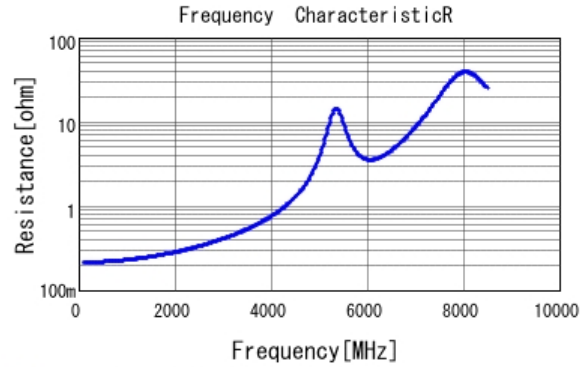
■ GCM1885C1H8R0DA16 R DCOV, 25degC
