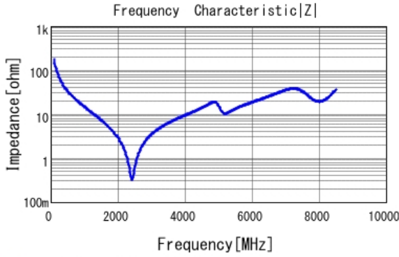
■ GCM1885C1H9R0BA16 |Z| DCOV, 25degC
