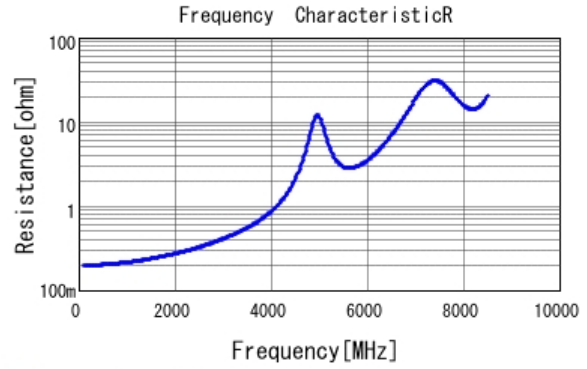
■ GCM1885C1H9R0BA16 R DCOV, 25degC
