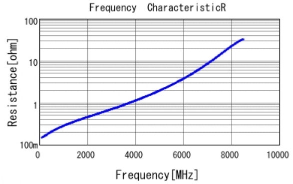
■ GCM1885C2A150JA16 R DCOV, 25degC
