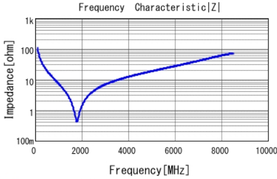
■ GCM1885C2A150JA16 |Z| DCOV, 25degC
