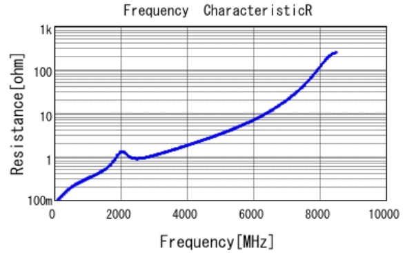
■ GCM1885C2A560JA16 R DCOV, 25degC
