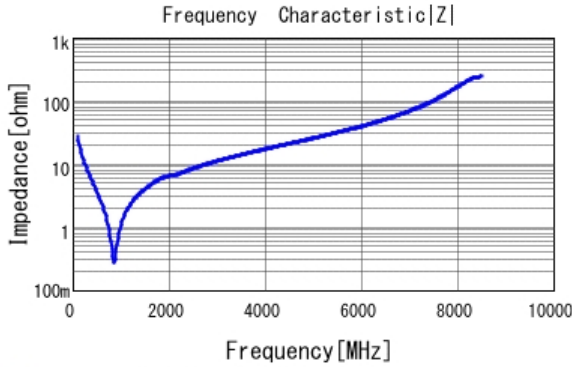
■ GCM1885C2A560JA16 |Z| DCOV, 25degC
