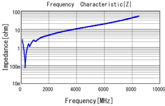
■ GCM1885C2A561JA16 |Z| DCOV, 25degC
