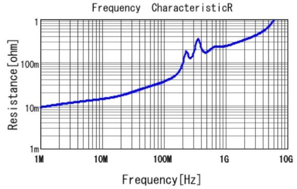
■ GCM1887U2A472JA16 R DCOV, 25degC
