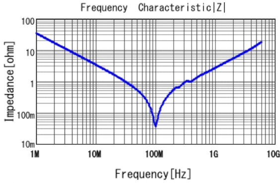
■ GCM1887U2A472JA16 |Z| DCOV, 25degC
