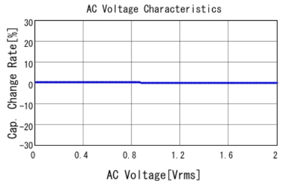
■ GCM1887U2A472JA16 C-AC Voltage capchange, DCOV, 25.0d
