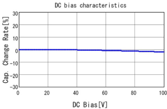
■ GCM1887U2A472JA16 C-DC bias capchange, 25.0degC, AC1V
