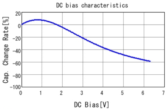
GCM188R70J225KE22 C-DC bias capchange, 25.0degC, AC0.
