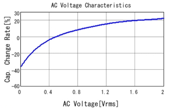
GCM188R70J225KE22 C-AC Voltage capchange, DCOV, 25.0d
