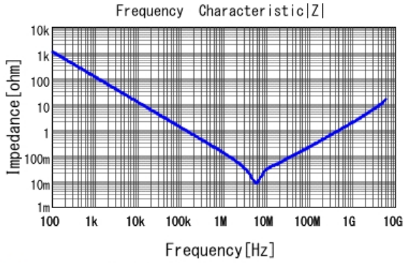
GCM188R70J225KE22 |Z| DCOV, 25degC
