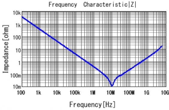
GCM188R71C474KA55 |Z| DCOV, 25degC
