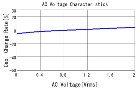
GCM188R71C474KA55 C-AC Voltage capchange, DCOV, 25.0d
