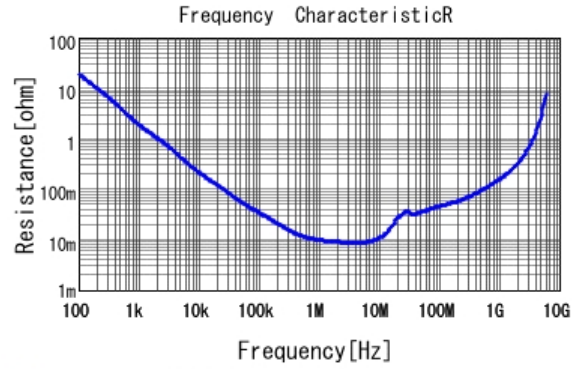
GCM188R71C474KA55 R DCOV, 25degC
