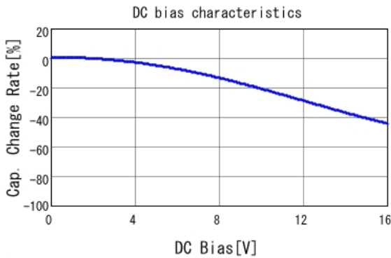
GCM188R71C474KA55 C-DC bias capchange, 25.0degC, AC1.
