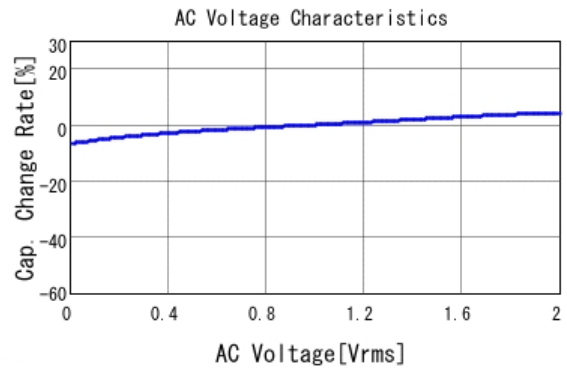
GCM188R71E102KA37 C-AC Voltage capchange, DCOV, 25.0d
