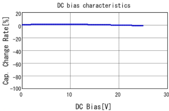
GCM188R71E102KA37 C-DC bias capchange, 25.0degC, AC1.
