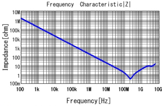
GCM188R71E102KA37 |Z| DCOV, 25degC
