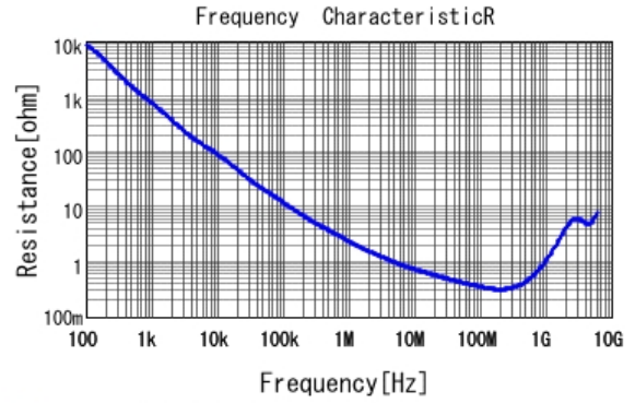
GCM188R71E102KA37 R DCOV, 25degC
