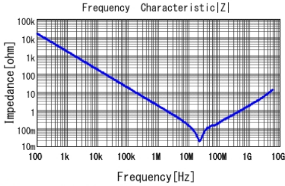
GCM188R71E104KA57 |Z| DCOV, 25degC
