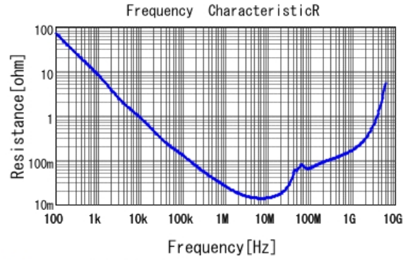
GCM188R71E104KA57 R DCOV, 25degC
