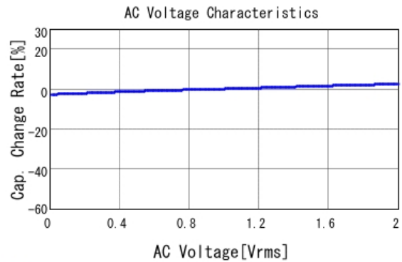
GCM188R71E104KA57 C-AC Voltage capchange, DCOV, 25.0d
