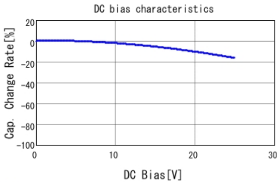
GCM188R71E104KA57 C-DC bias capchange, 25.0degC, AC1.
