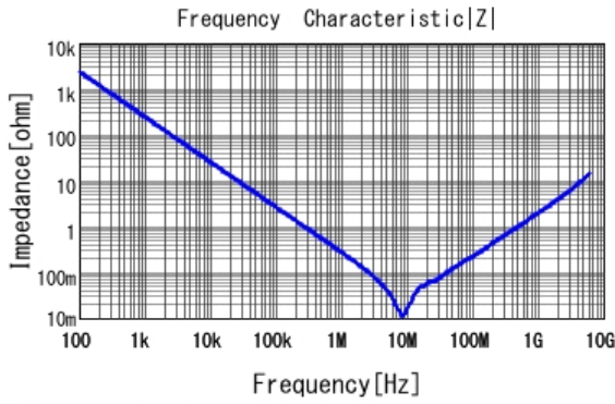
GCM188R71E105KA64 |Z| DC0V, 25degC
