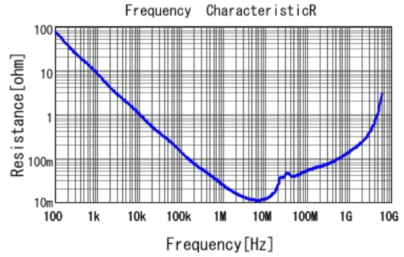
GCM188R71E474KA64 R DCOV, 25degC
