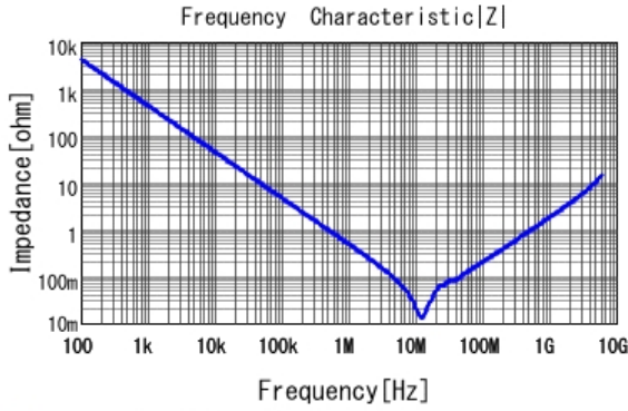
GCM188R71E474KA64 |Z| DCOV, 25degC
