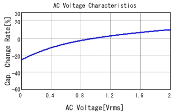
GCM188R71E474KA64 C-AC Voltage capchange, DCOV, 25.0d
