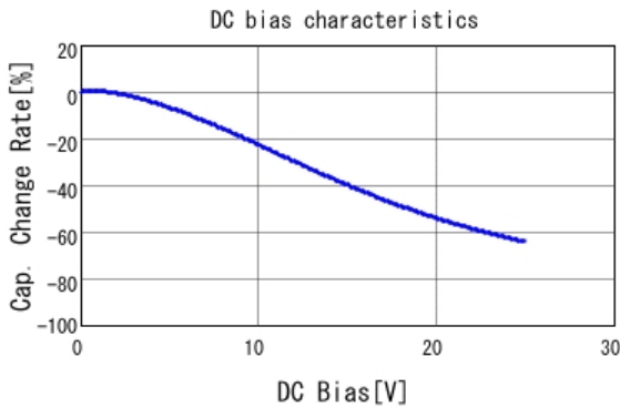
GCM188R71E474KA64 C-DC bias capchange, 25.0degC, AC1.
