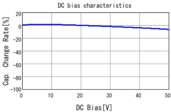
GCM188R71H102KA37 C-DC bias capchange, 25.0degC, AC1.
