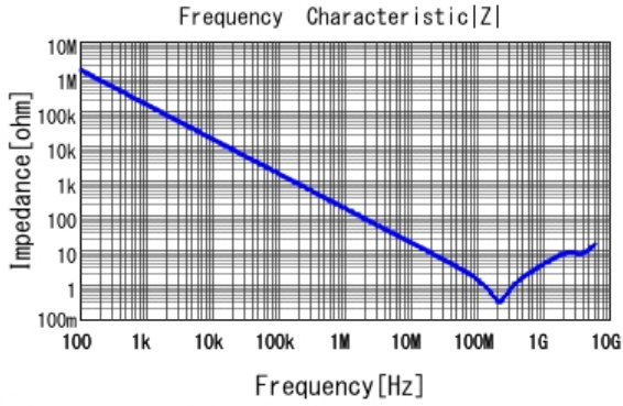
GCM188R71H102KA37 |Z| DCOV, 25degC
