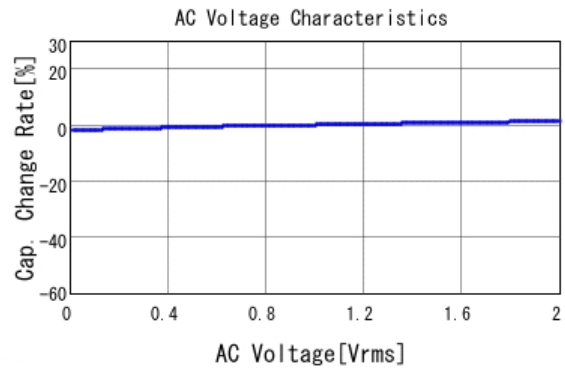
GCM188R71H102KA37 C-AC Voltage capchange, DCOV, 25.0d
