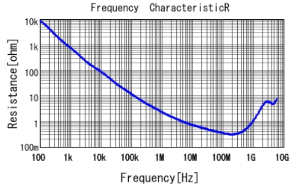
GCM188R71H102KA37 R DCOV, 25degC
