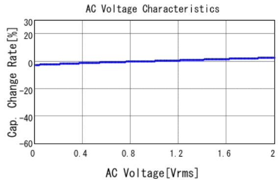
■ GCM188R71H104KA57 C-AC Voltage capchange, DCOV, 25.0d
