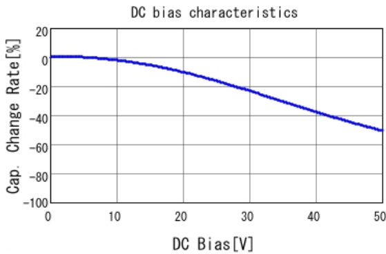
■ GCM188R71H104KA57 C-DC bias capchange, 25.0degC, AC1.
