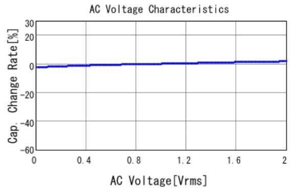
GCM188R71H153KA37 C-AC Voltage capchange, DCOV, 25.0d
