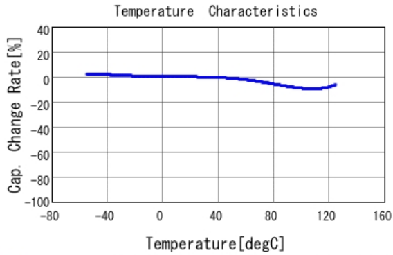
■ GCM188R71H153KA37 C-Temp. capchange, DC0.0V, AC1.0V rm
