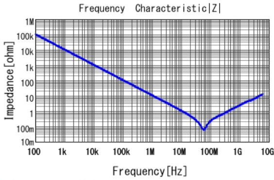
GCM188R71H153KA37 |Z| DCOV, 25degC
