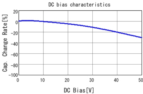
GCM188R71H153KA37 C-DC bias capchange, 25.0degC, AC1.
