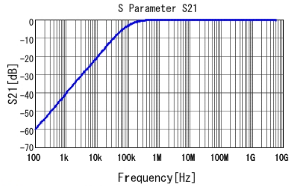
■ GCM188R71H153KA37 S21 DC0V, 25degC
