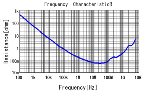
GCM188R71H153KA37 R DCOV, 25degC
