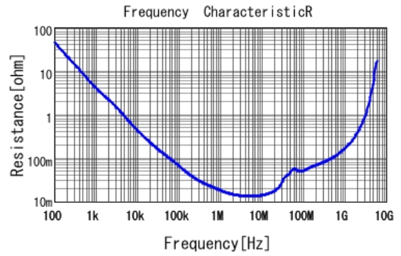
GCM188R71H154KA64 R DC0V, 25degC
