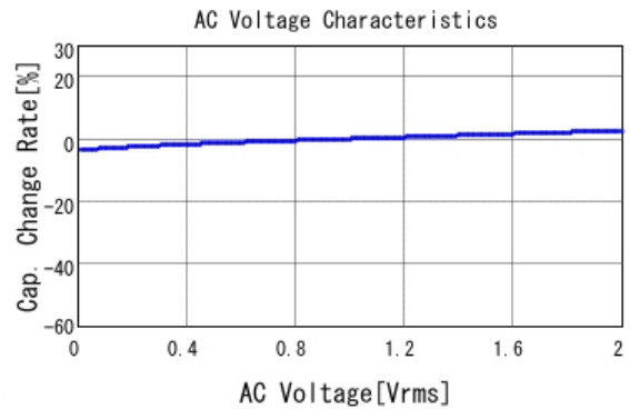
GCM188R71H154KA64 C-AC Voltage capchange, DC0V, 25.0d
