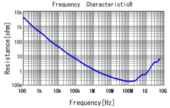
GCM188R71H222KA37 R DCOV, 25degC
