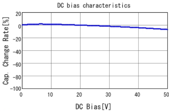
GCM188R71H222KA37 C-DC bias capchange, 25.0degC, AC1.
