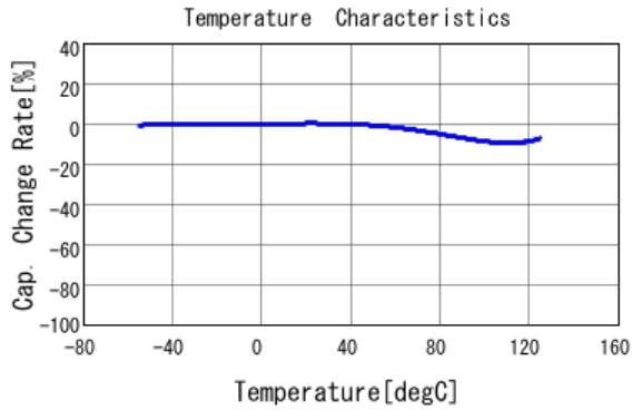
■ GCM188R71H222KA37 C-Temp. capchange, DC0.0V, AC1.0V rm
