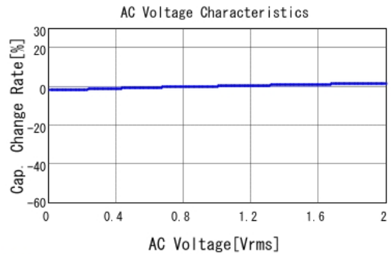
GCM188R71H222KA37 C-AC Voltage capchange, DCOV, 25.0d
