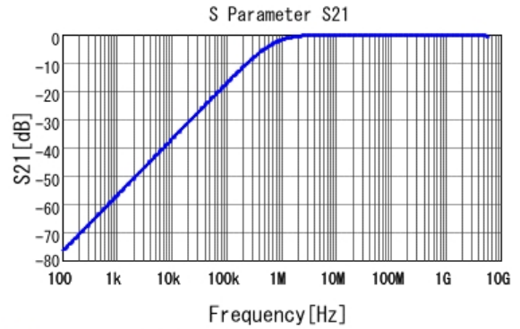
■ GCM188R71H222KA37 S21 DC0V, 25degC
