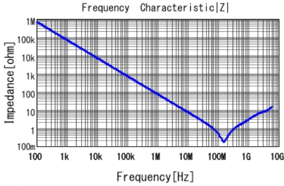
GCM188R71H222KA37 |Z| DCOV, 25degC
