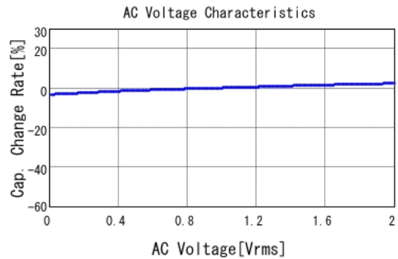
GCM188R71H224KA64 C-AC Voltage capchange, DCOV, 25.0d
