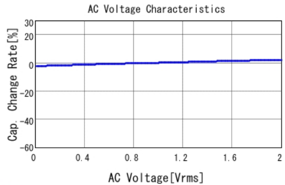
GCM188R71H333KA55 C-AC Voltage capchange, DCOV, 25.0d
