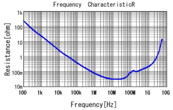
GCM188R71H333KA55 R DCOV, 25degC
