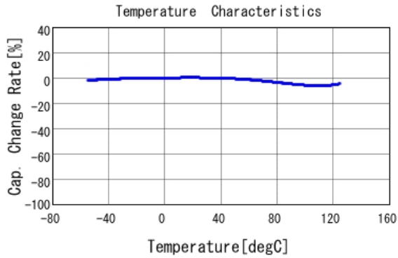
■ GCM188R71H333KA55 C-Temp. capchange, DC0.0V, AC1.0V rms
