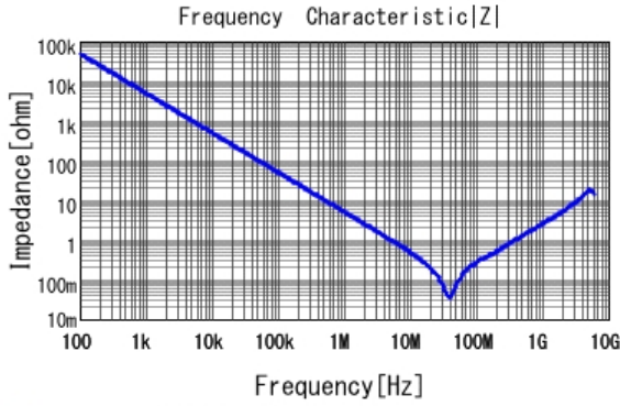
GCM188R71H333KA55 |Z| DCOV, 25degC
