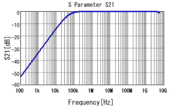
■ GCM188R71H333KA55 S21 DC0V, 25degC
