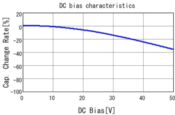
GCM188R71H333KA55 C-DC bias capchange, 25.0degC, AC1.
