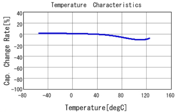
■ GCM188R71H682KA37 C-Temp. capchange, DC0.0V, AC1.0V rm
