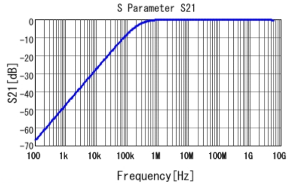
■ GCM188R71H682KA37 S21 DC0V, 25degC
