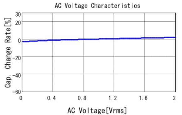
GCM188R72A103KA37 C-AC Voltage capchange, DCOV, 25.0d
