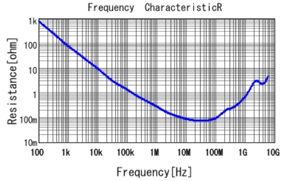
GCM188R72A103KA37 R DCOV, 25degC
