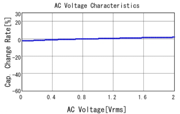
GCM188R72A472KA37 C-AC Voltage capchange, DCOV, 25.0d
