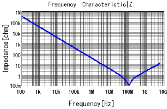
GCM188R72A472KA37 |Z| DCOV, 25degC
