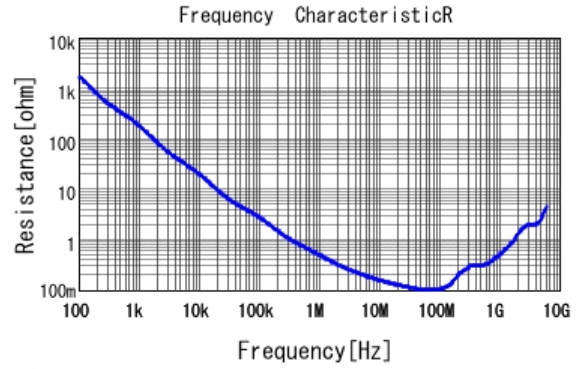
GCM188R72A472KA37 R DCOV, 25degC
