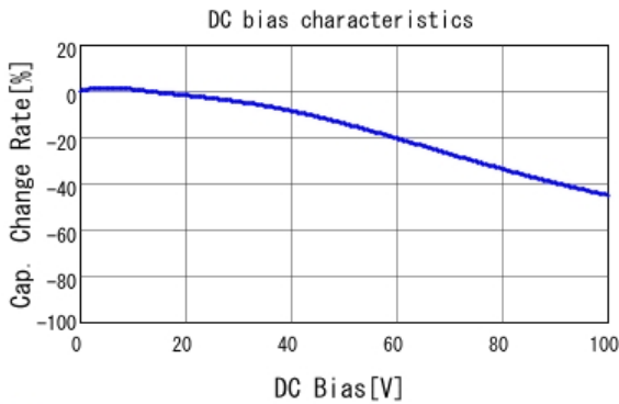
GCM188R72A472KA37 C-DC bias capchange, 25.0degC, AC1.
