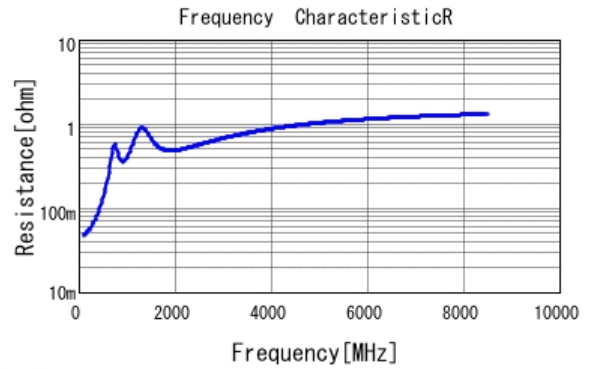
■ GCM2165C1H681JA16 R DCOV, 25degC
