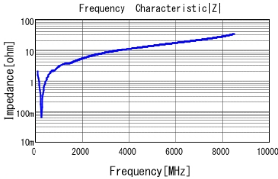
■ GCM2165C1H681JA16 |Z| DCOV, 25degC
