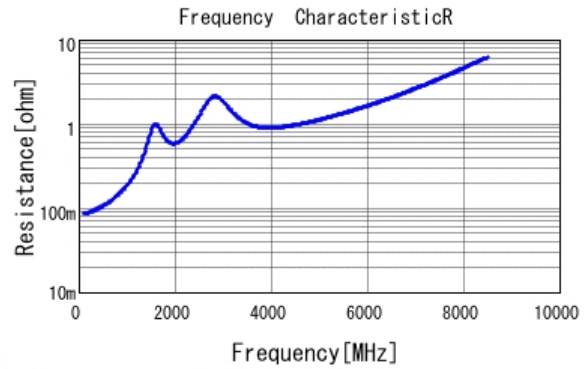
■ GCM2165C2A181JA16 R DC0V, 25degC
