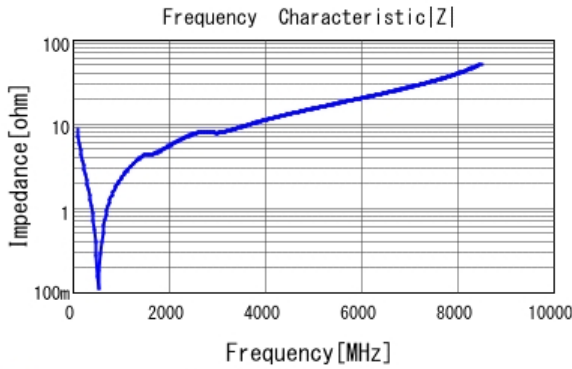
■ GCM2165C2A181JA16 |Z| DC0V, 25degC
