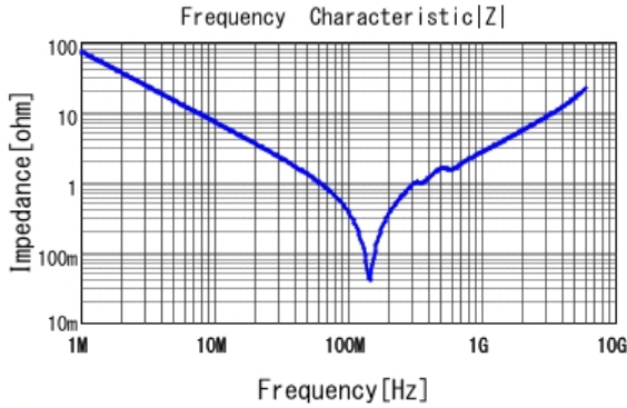
■ GCM2165C2A222JA16 |Z| DCOV, 25degC
