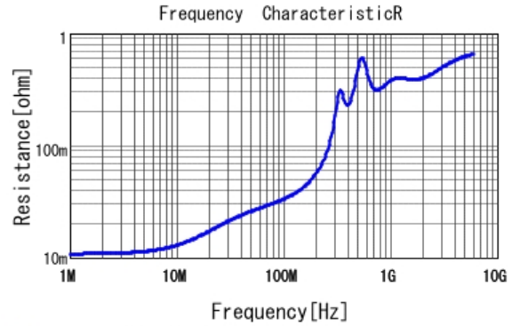
■ GCM2165C2A222JA16 R DCOV, 25degC
