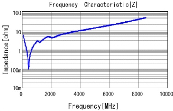
■ GCM2165C2A271JA16 |Z| DCOV, 25degC
