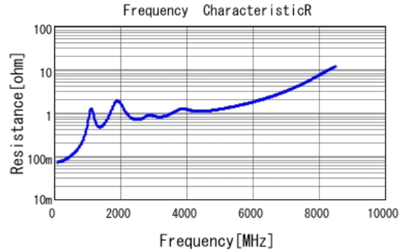
■ GCM2165C2A271JA16 R DCOV, 25degC
