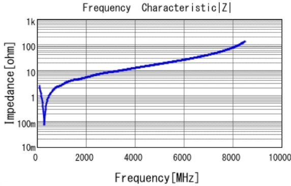
■ GCM2165C2A561JA16 |Z| DCOV, 25degC
