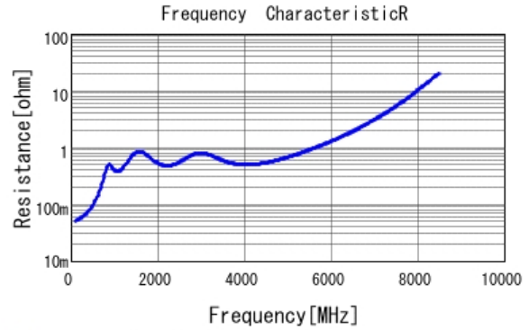
■ GCM2165C2A561JA16 R DCOV, 25degC
