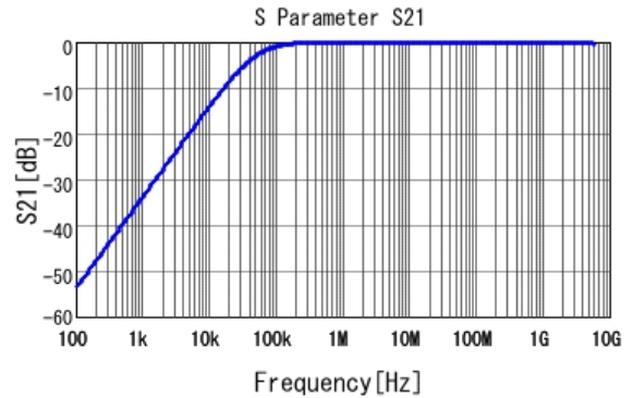
■ GCM219R71H333KA37 S21 DC0V, 25degC
