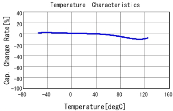
■ GCM219R71H333KA37 C-Temp. capchange, DC0.0V, AC1.0V rm
