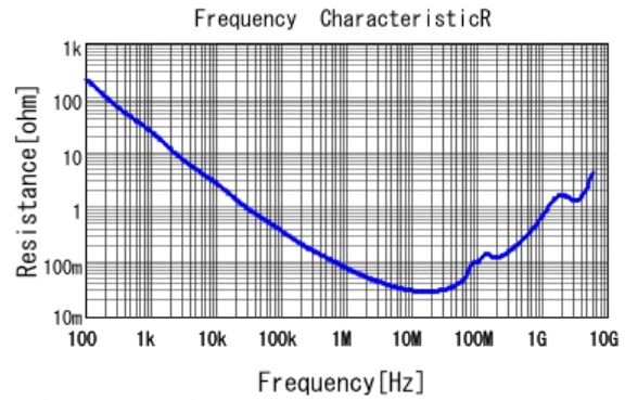
GCM219R72A333KA37 R DCOV, 25degC
