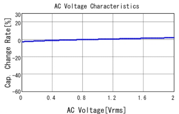
GCM219R72A333KA37 C-AC Voltage capchange, DCOV, 25.0d
