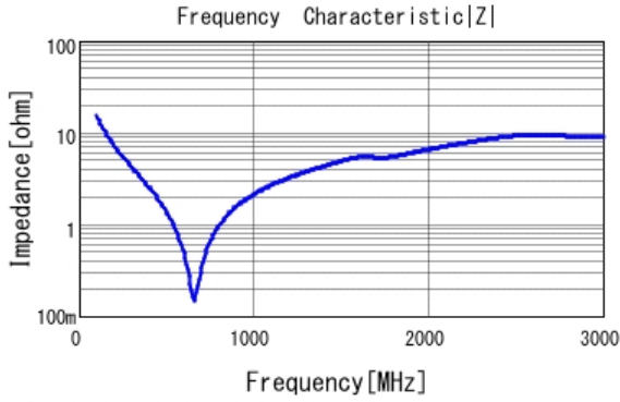
■ GCM21A5C2E101JX01 |Z| DC0V, 25degC
