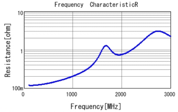
■ GCM21A5C2E101JX01 R DC0V, 25degC
