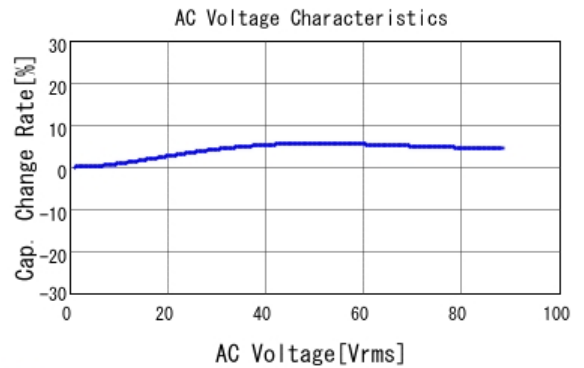
■ GCM21A7U2E151JX01 C-AC Voltage capchange, DC0V, 25.0d
