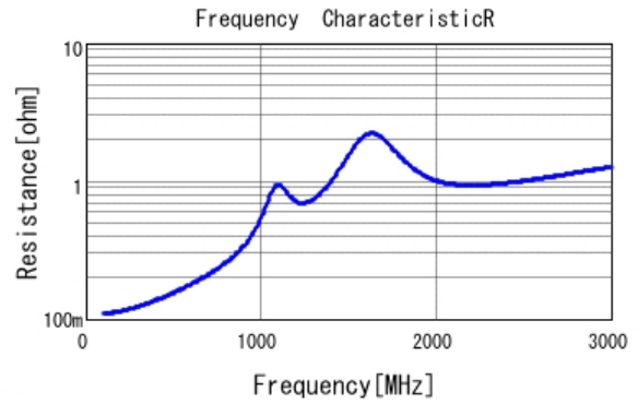
■ GCM21A7U2E151JX01 R DC0V, 25degC
