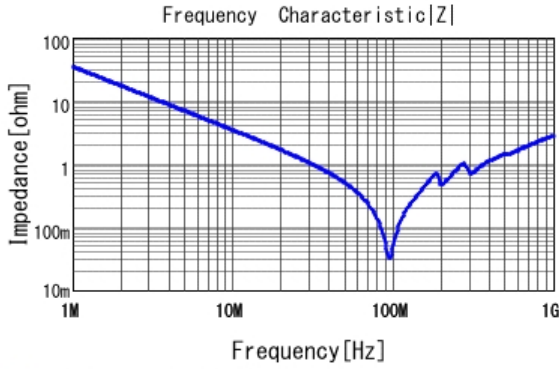
■ GCM21B5C2E472JX01 |Z| DC0V, 25degC
