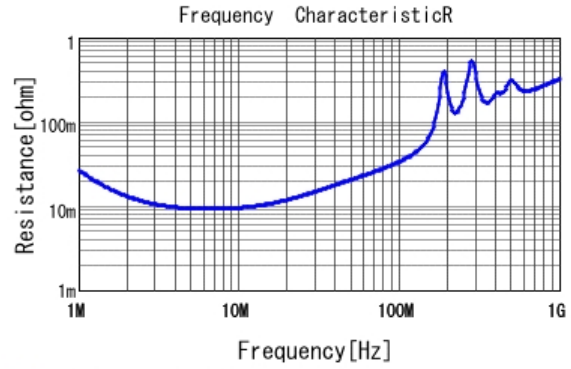
■ GCM21B5C2E472JX01 R DC0V, 25degC
