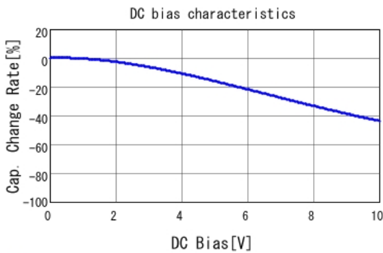
GCM21BC71A475KA73 C-DC bias capchange, 25.0degC, AC1.
