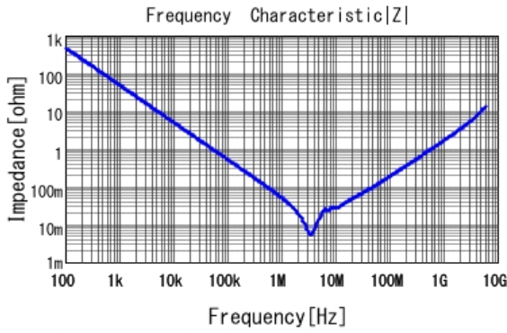
GCM21BC71A475KA73 |Z| DC0V, 25degC
