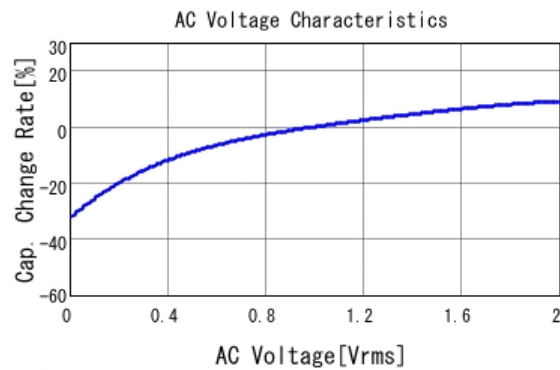
GCM21BC71A475KA73 C-AC Voltage capchange, DC0V, 25.0d
