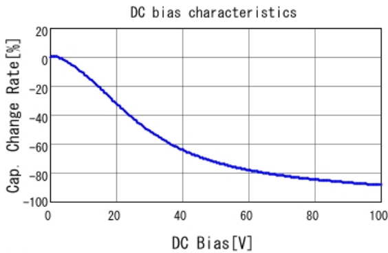
GCM21BC72A105KE36 C-DC bias capchange, 25.0degC, AC1.
