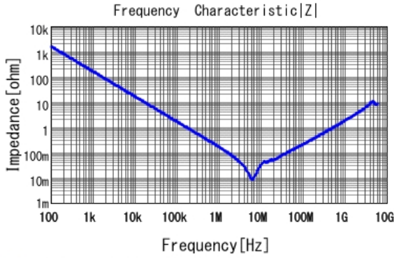
GCM21BC72A105KE36 |Z| DC0V, 25degC
