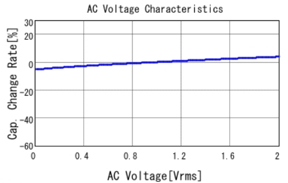
GCM21BC72A105KE36 C-AC Voltage capchange, DC0V, 25.0d
