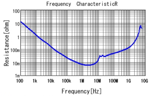
GCM21BC72A105KE36 R DC0V, 25degC
