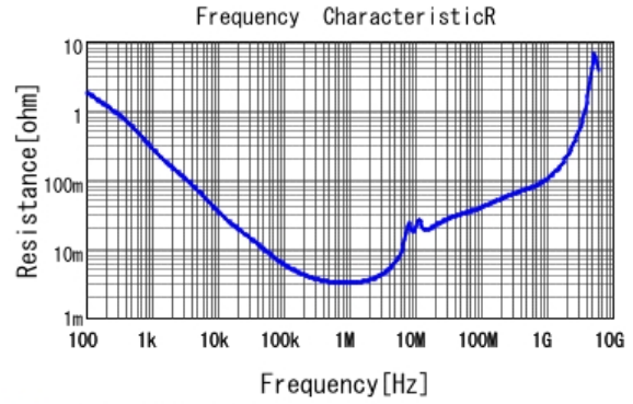
GCM21BC7YA225KE02 R DC0V, 25degC
