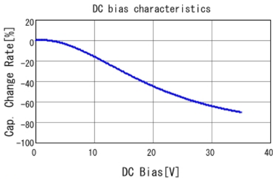
GCM21BC7YA225KE02 C-DC bias capchange, 25.0degC, AC1.
