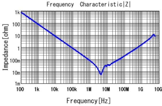
GCM21BC7YA225KE02 |Z| DC0V, 25degC
