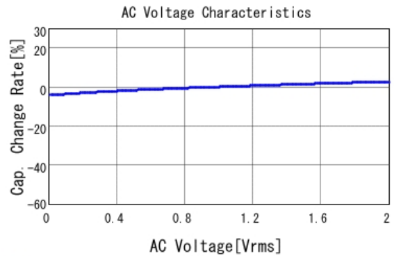
GCM21BC7YA225KE02 C-AC Voltage capchange, DC0V, 25.0d
