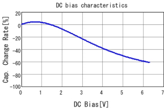
■ GCM21BR70J106KE22 C-DC bias capchange, 25.0degC, AC0.
