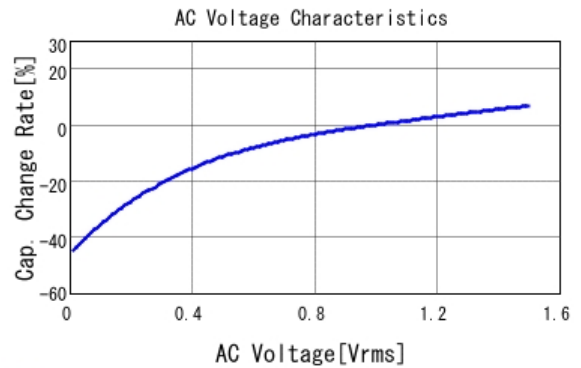
GCM21BR71A106KE22 C-AC Voltage capchange, DC0V, 25.0d
