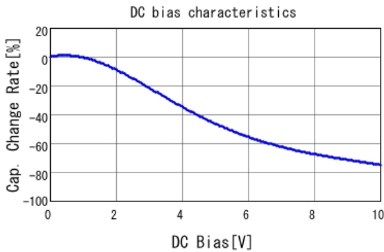
GCM21BR71A106KE22 C-DC bias capchange, 25.0degC, AC1V
