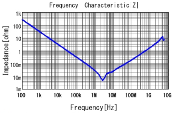
GCM21BR71A106KE22 |Z| DC0V, 25degC
