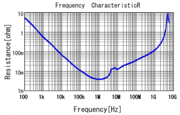
GCM21BR71A106KE22 R DC0V, 25degC
