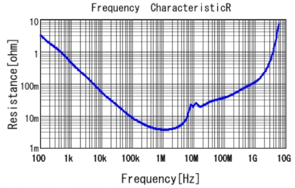
■ GCM21BR71A225KA37 R DCOV, 25degC
