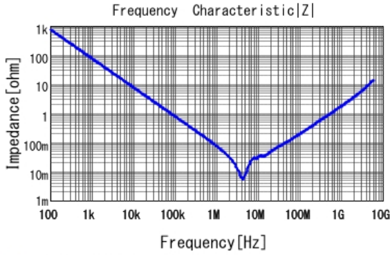
■ GCM21BR71A225KA37 |Z| DCOV, 25degC
