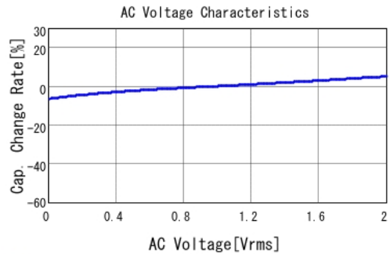
■ GCM21BR71A225KA37 C-AC Voltage capchange, DCOV, 25.0d
