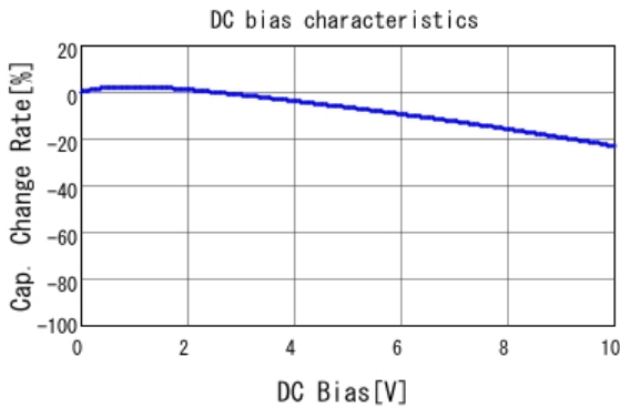
■ GCM21BR71A225KA37 C-DC bias capchange, 25.0degC, AC1.
