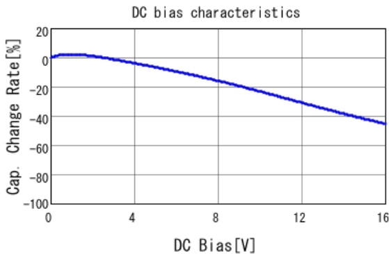
GCM21BR71C225KA64 C-DC bias capchange, 25.0degC, AC1.
