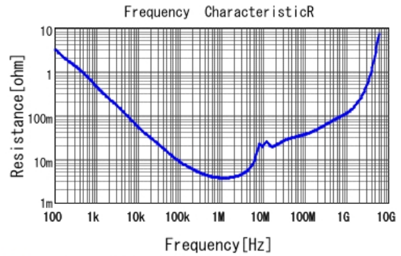
GCM21BR71C225KA64 R DC0V, 25degC
