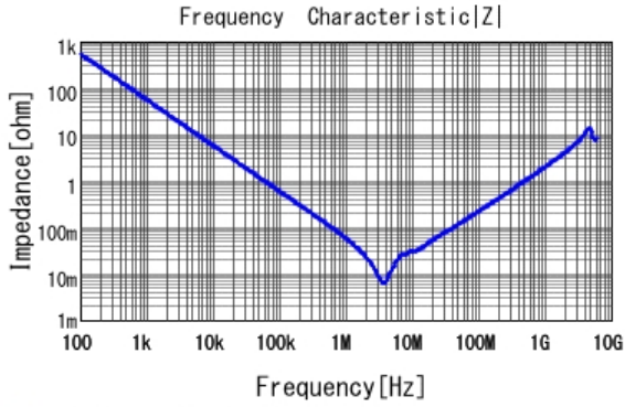
■ GCM21BR71C475KA73 |Z| DC0V, 25degC
