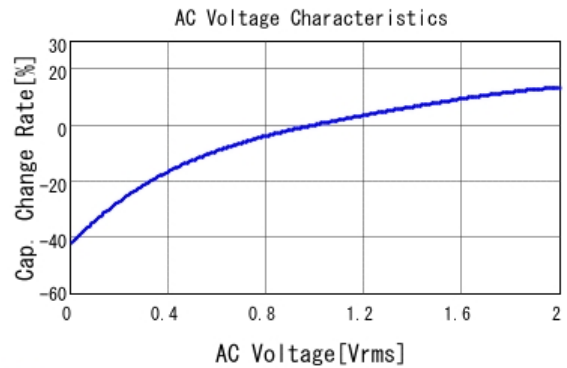
■ GCM21BR71C475KA73 C-AC Voltage capchange, DC0V, 25.0d
