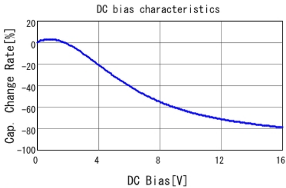
■ GCM21BR71C475KA73 C-DC bias capchange, 25.0degC, AC1.
