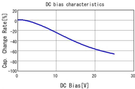
■ GCM21BR71E225KA73 C-DC bias capchange, 25.0degC, AC1.
