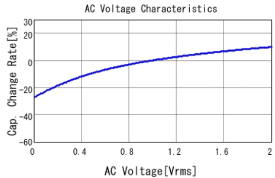
■ GCM21BR71E225KA73 C-AC Voltage capchange, DCOV, 25.0d
