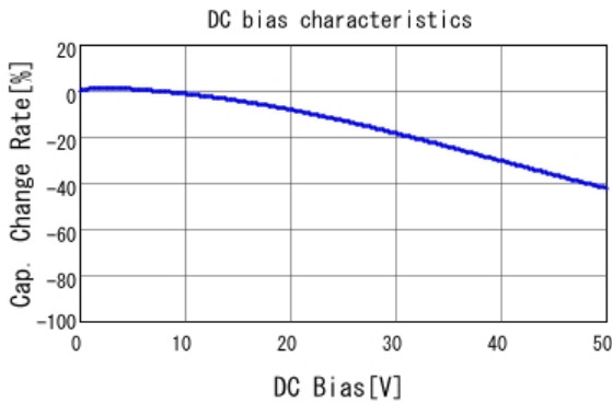
GCM21BR71H104KA37 C-DC bias capchange, 25.0degC, AC1.
