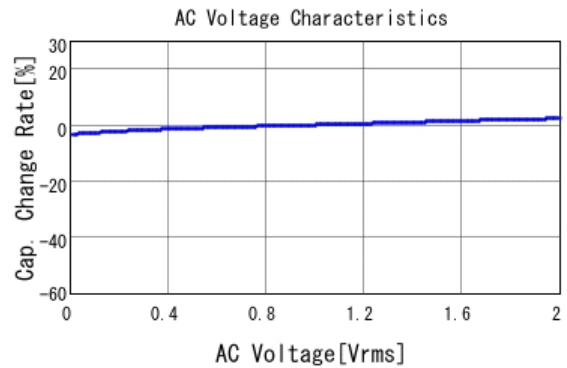
GCM21BR71H104KA37 C-AC Voltage capchange, DCOV, 25.0d
