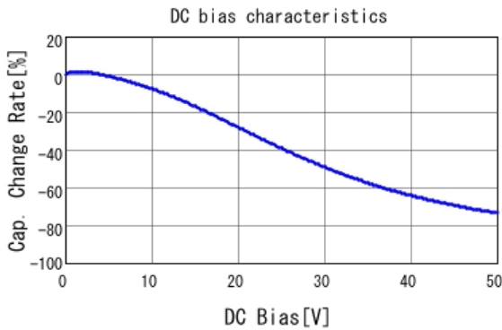
GCM21BR71H105KA03 C-DC bias capchange, 25.0degC, AC1.
