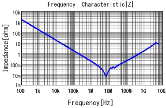
GCM21BR71H105KA03 |Z| DC0V, 25degC
