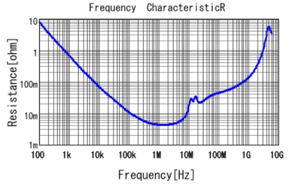
GCM21BR71H105KA03 R DC0V, 25degC
