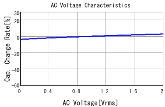
GCM21BR71H105KA03 C-AC Voltage capchange, DC0V, 25.0d
