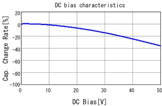
■ GCM21BR71H154KA37 C-DC bias capchange, 25.0degC, AC1.
