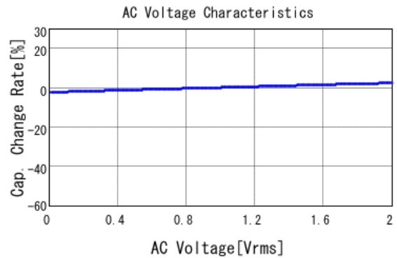
■ GCM21BR71H154KA37 C-AC Voltage capchange, DC0V, 25.0d
