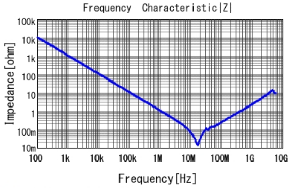
■ GCM21BR71H154KA37 |Z| DC0V, 25degC
