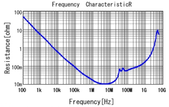
■ GCM21BR71H154KA37 R DC0V, 25degC
